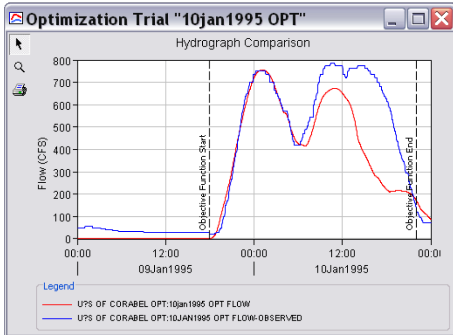
Figure 5. Calibration results for the January 10, 1995 event
