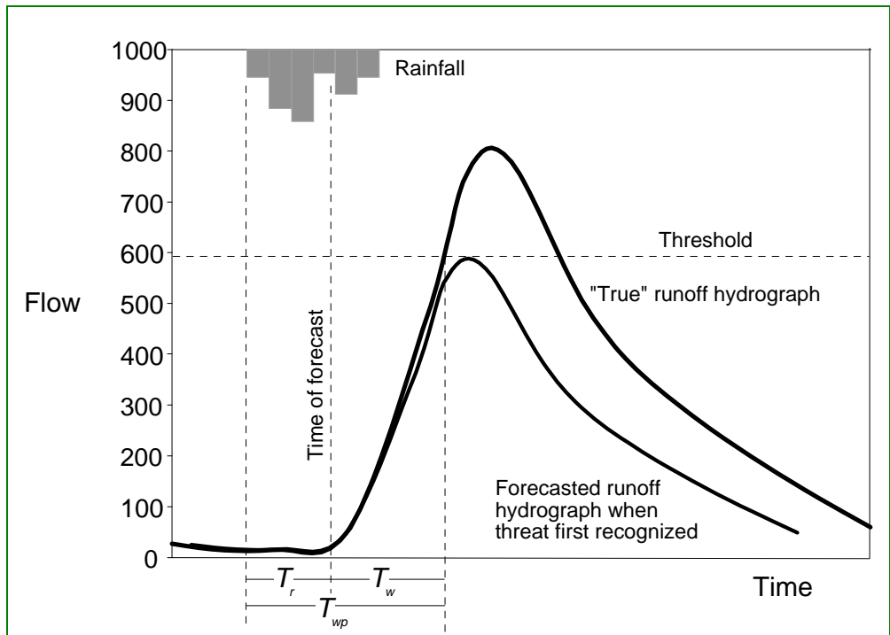
Figure 34. Warning time components
