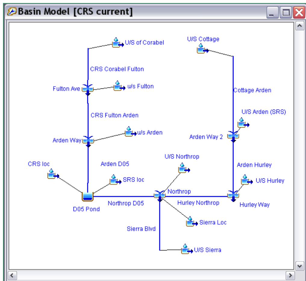
Figure 20. Complete basin model of CRS/SRS watershed
