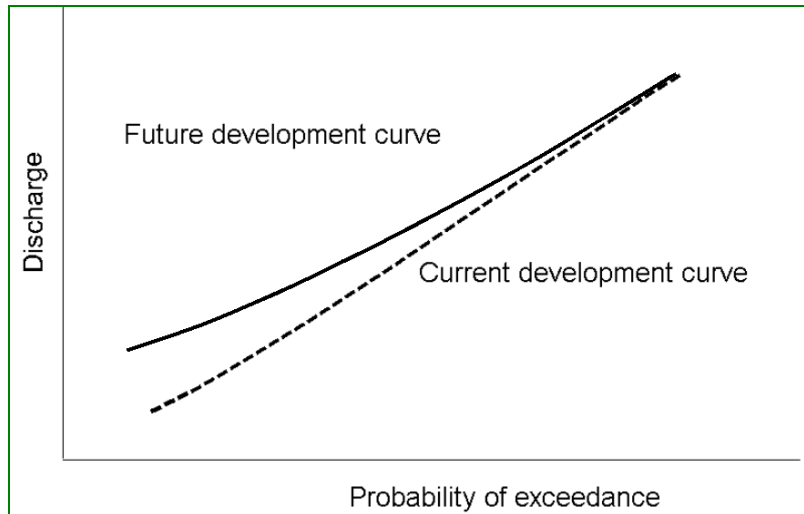
Figure 16. Comparison of without-project flow-frequency curves
