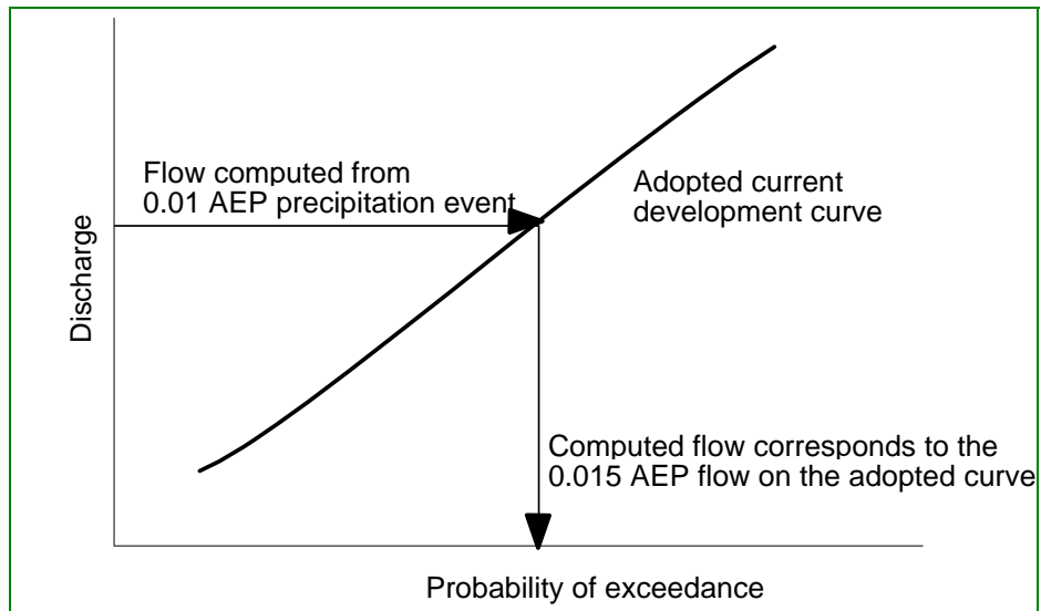
Figure 18. Example of using adopted frequency curve to assign AEP
